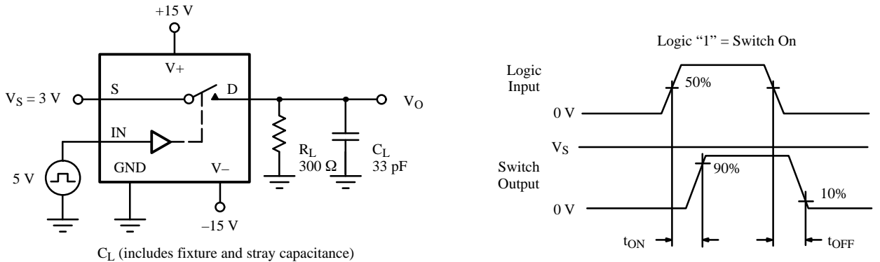
Figure 2. Switching Time
